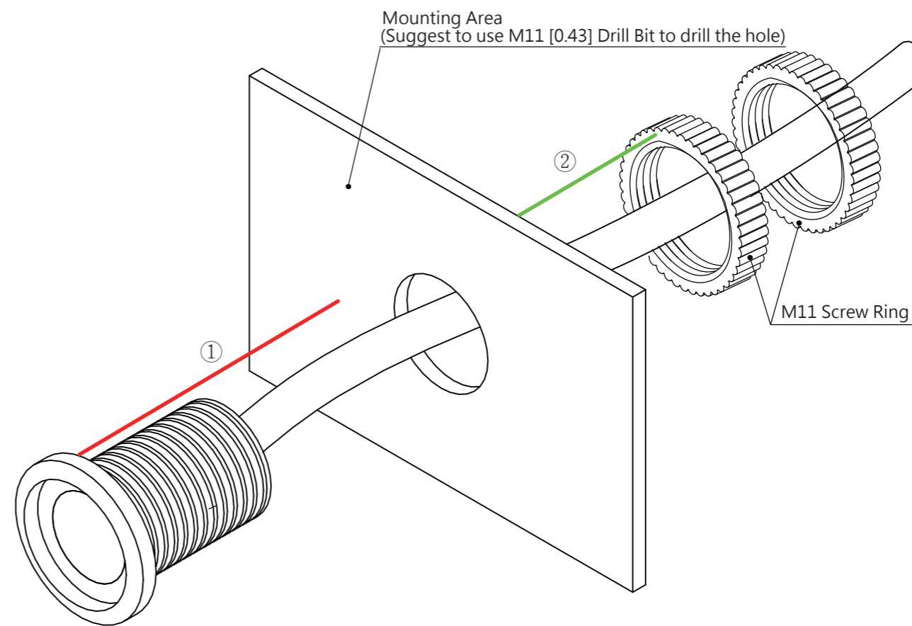
INSTALLATION DIAGRAM
