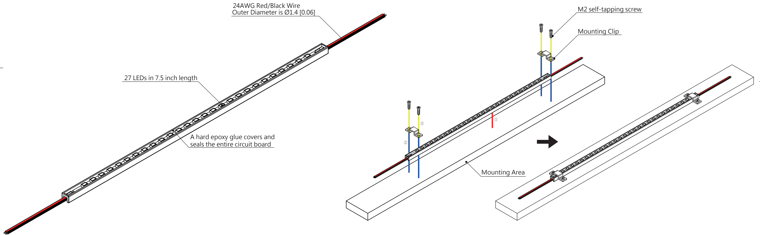
ISOMETRIC VIEW
