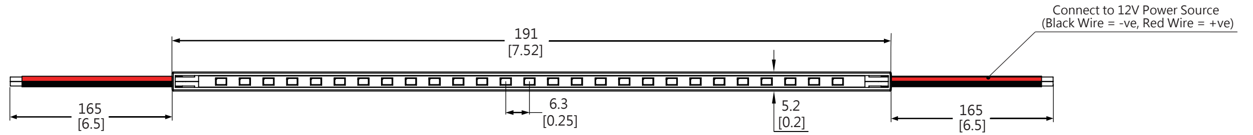
TOP VIEW
