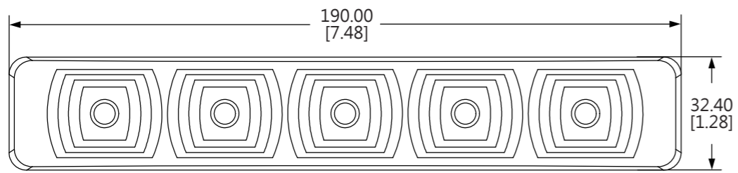
FRONT VIEW
