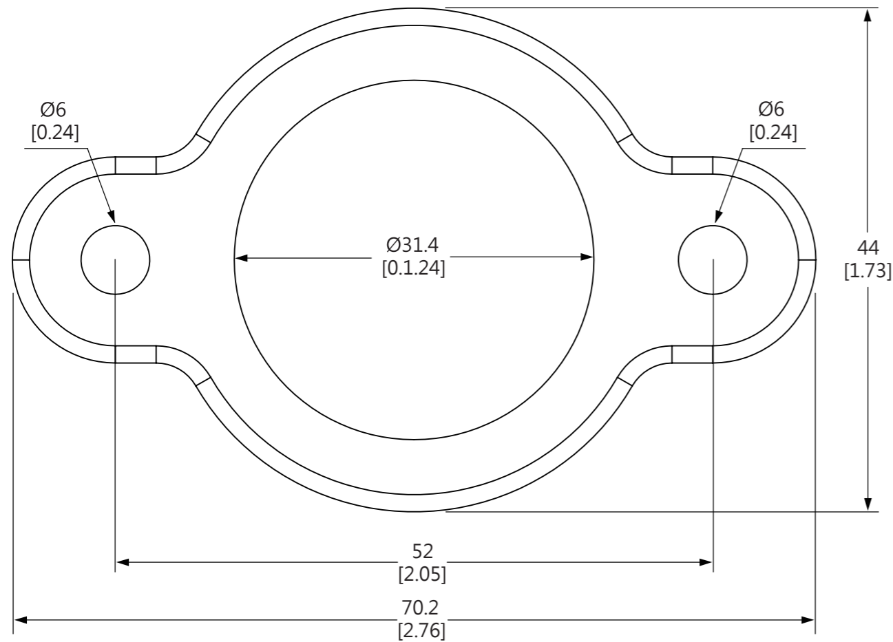
FRONT VIEW
